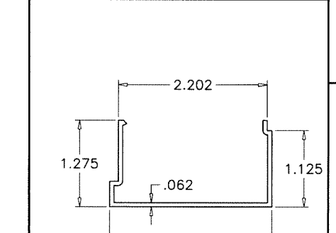
⑪ FEMALE MULLION
