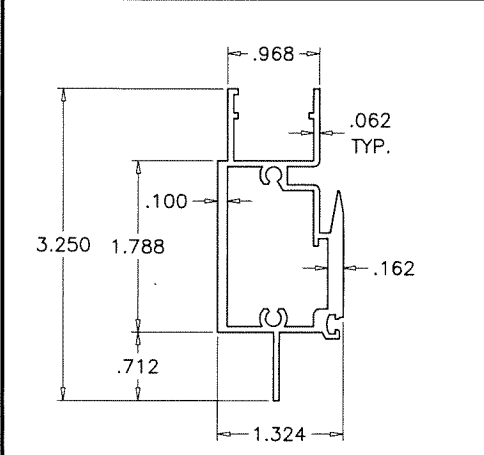
① FRAME HEAD/SILL
