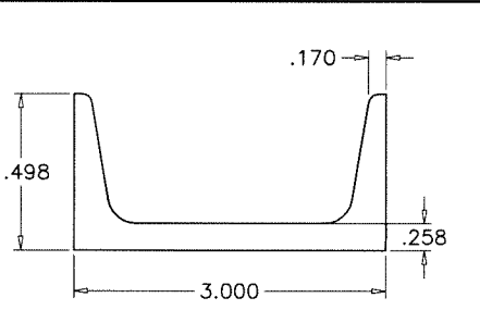
⑭ REINFORCING CHANNEL
