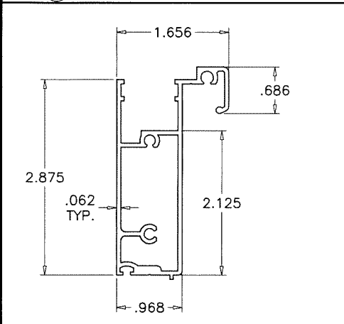
⑥ VENT BOTTOM RAIL
