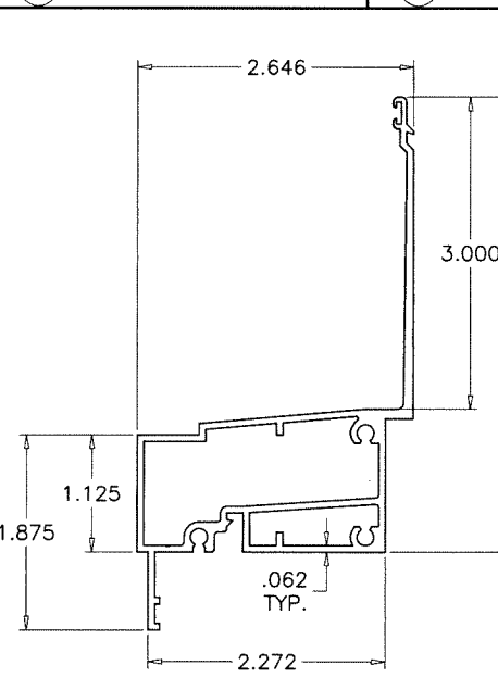
⑨ SILL MTG. RAIL W/ FIXED BOTTOM
