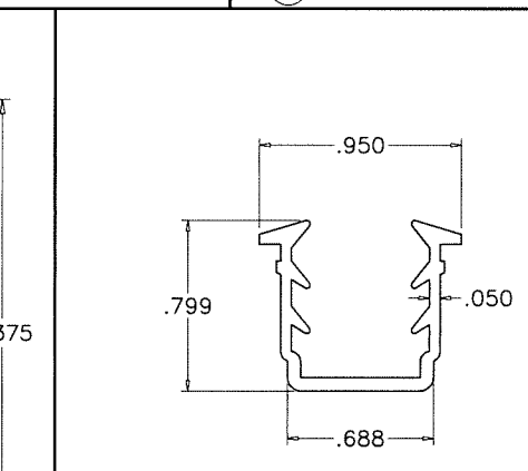
⑦ GLAZING BEAD
