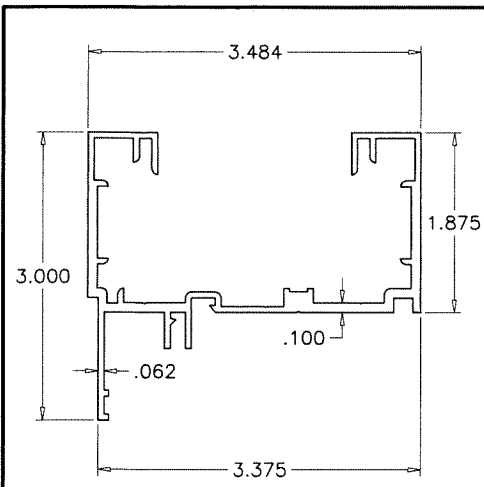
① FRAME HEAD/SILL
