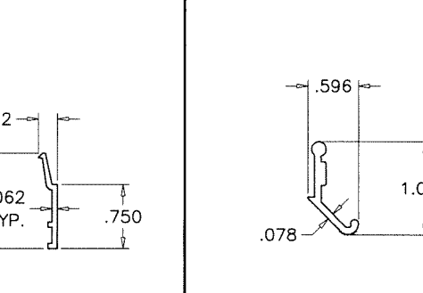
⑩ MALE MULLION
