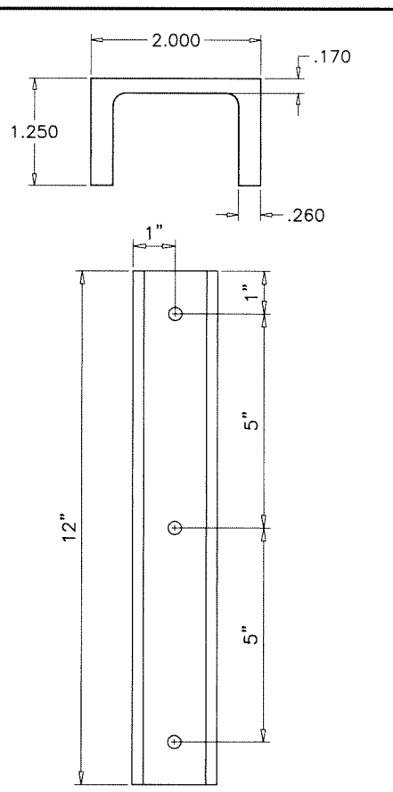
⑭ ANCHOR CHANNEL
