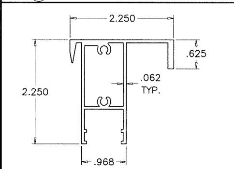
③ MEETING RAIL
