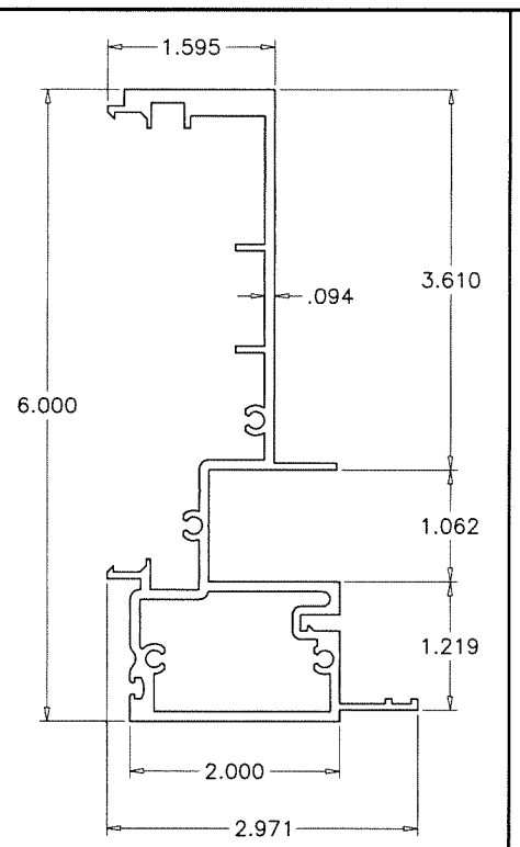
⑪ FEMALE MULLION
